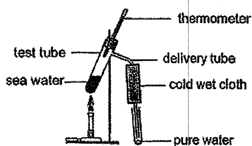
Set-up S
